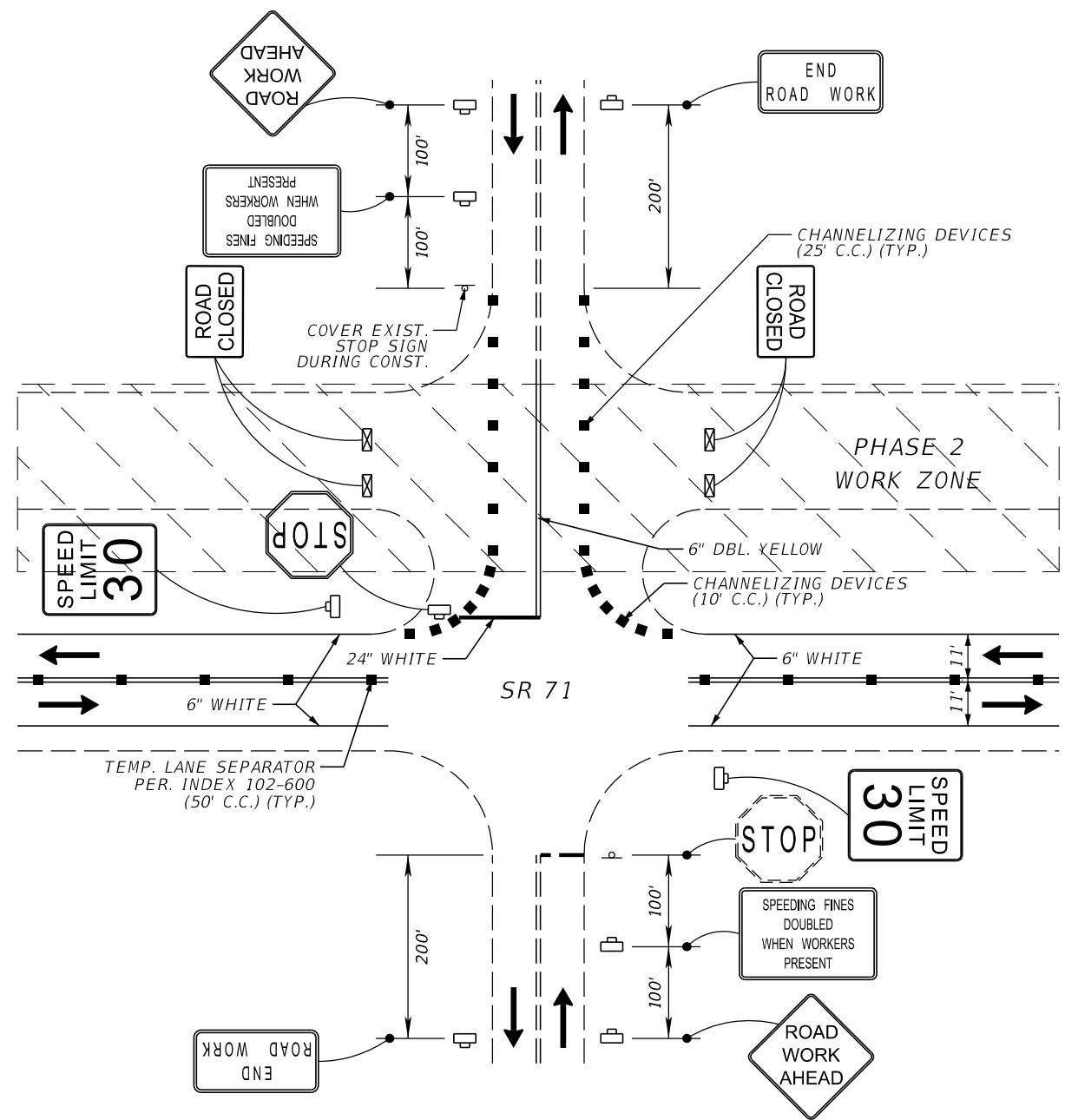
PHASE 2 SIDE STREET DETAIL N.T.S.
