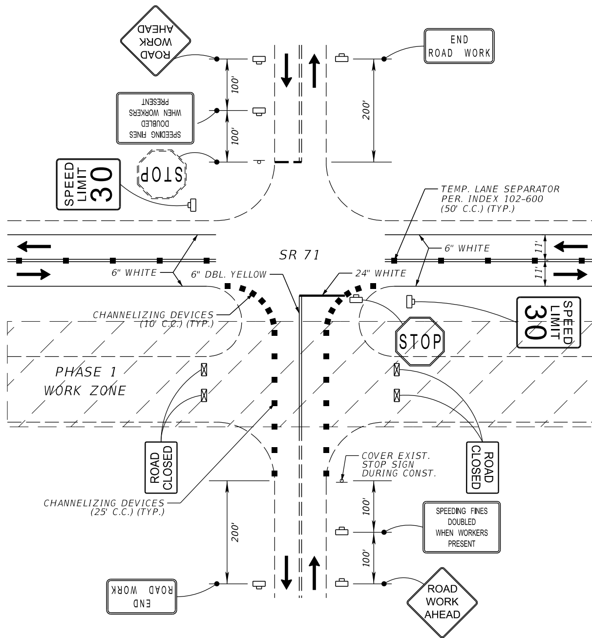
PHASE 1 SIDE STREET DETAIL N.T.S.
